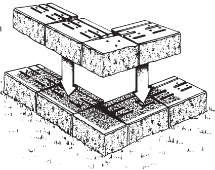
FIGURE 5 Outside 90° Corner
