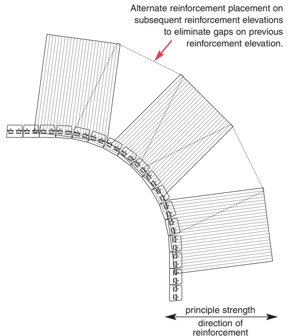
FIGURE 4 Concave Curve
