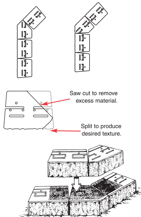
FIGURE 9 Large Angle Outside Corner
