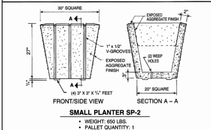
SMALL PLANTER SP-2 EXPOSED AGGREGATE #1 FINISH
