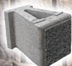
850 Half 8" h x 12" d x 9" l 45 block / cube .5 ft 2
