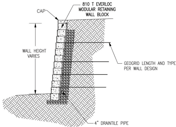
810 T RETAINING WALL DETAIL N.T.S.
