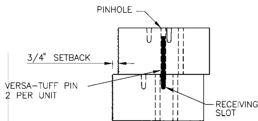
Pinning Detail
