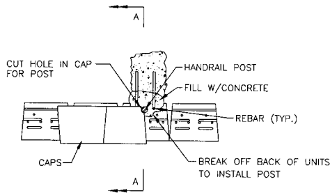
POST DETAIL- PLAN VIEW
