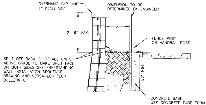
FREESTANDING WALL DETAIL (STRAIGHT WALLS ONLY)
