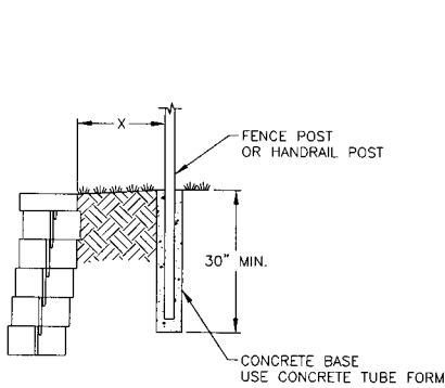
POST DETAIL
