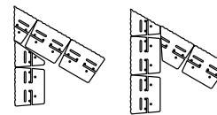
LOW-ANGLE, OUTSIDE
