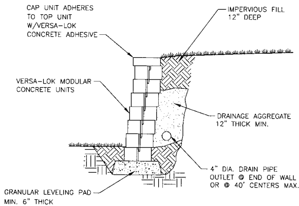
TYPICAL SECTION—UNREINFORCED RETAINING WALL
