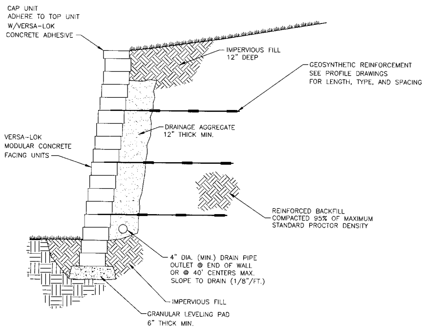
TYPICAL SECTION—REINFORCED RETAINING WALL
