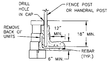
POST DETAIL- SECTION A-A
