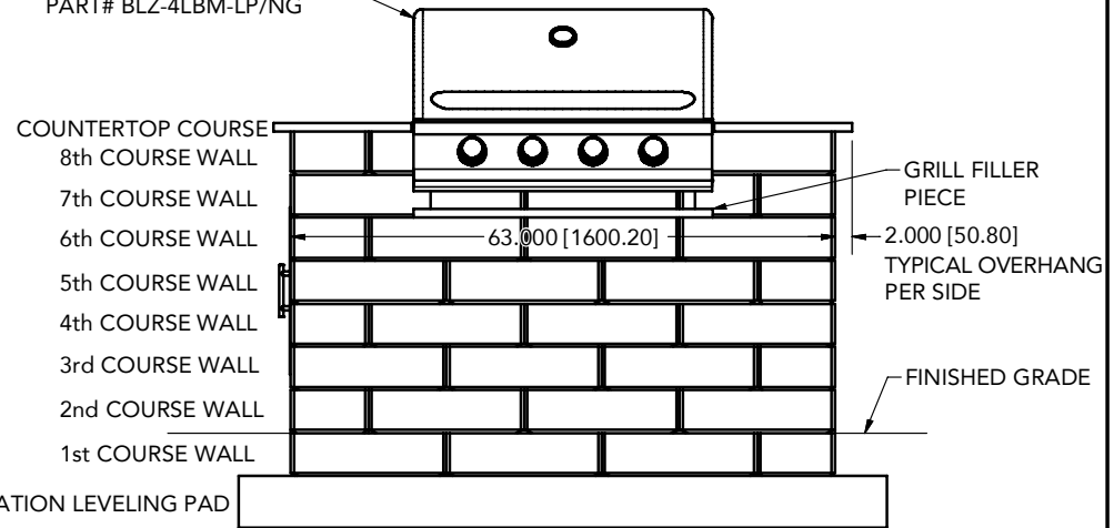
FRONT ELEVATION VIEW
