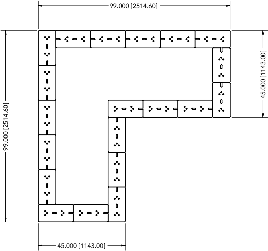
PLAN VIEW
