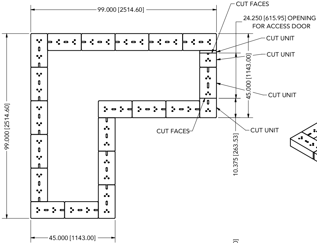
PLAN VIEW
