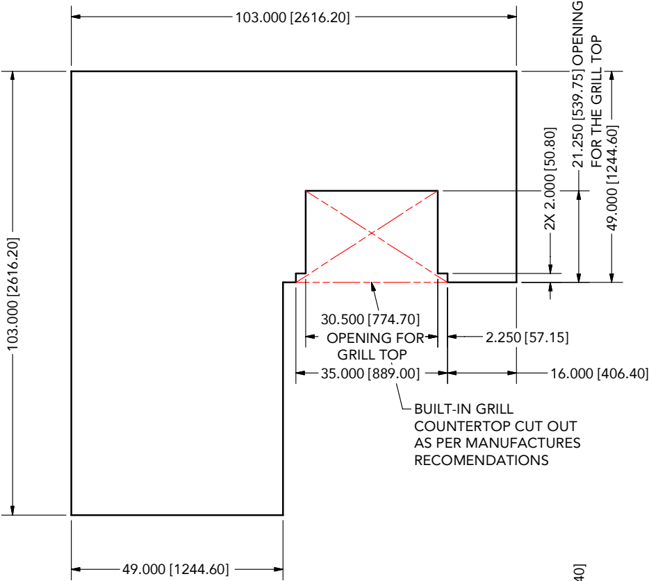
PLAN VIEW
