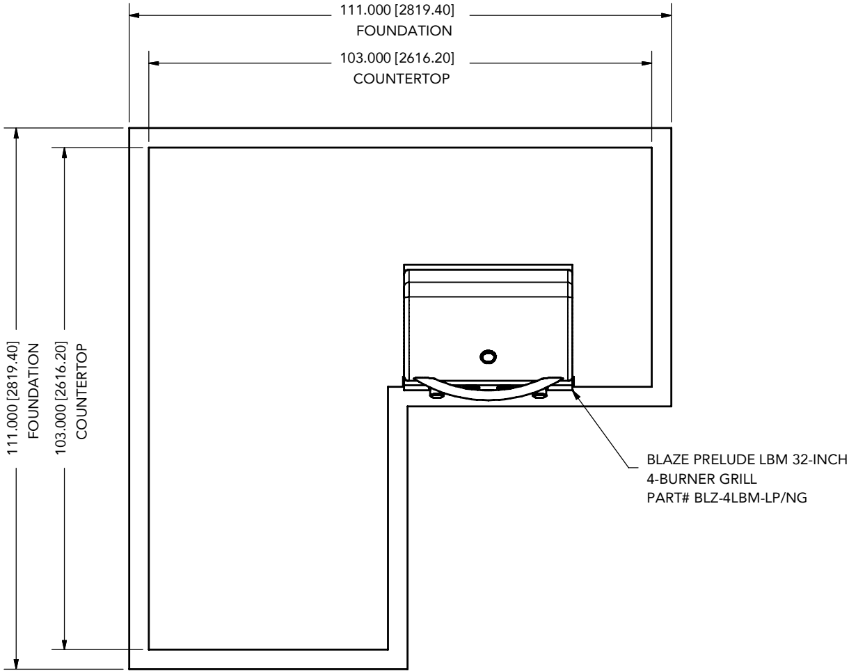
PLAN VIEW
