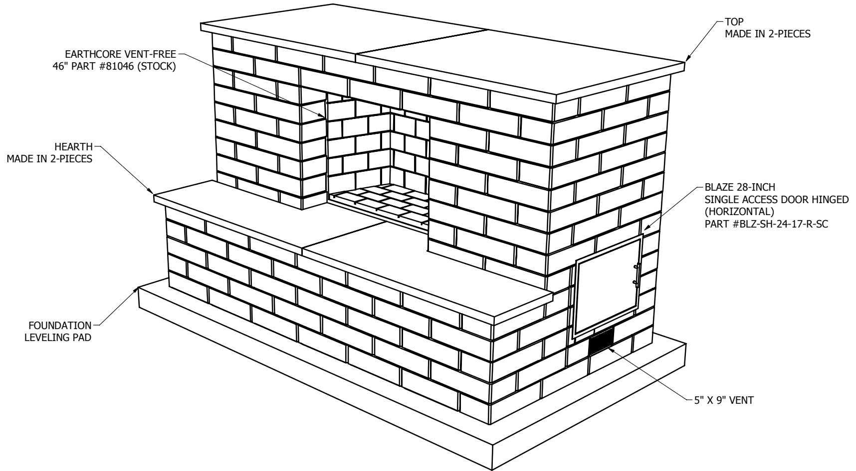
ISOMETRIC VIEW
