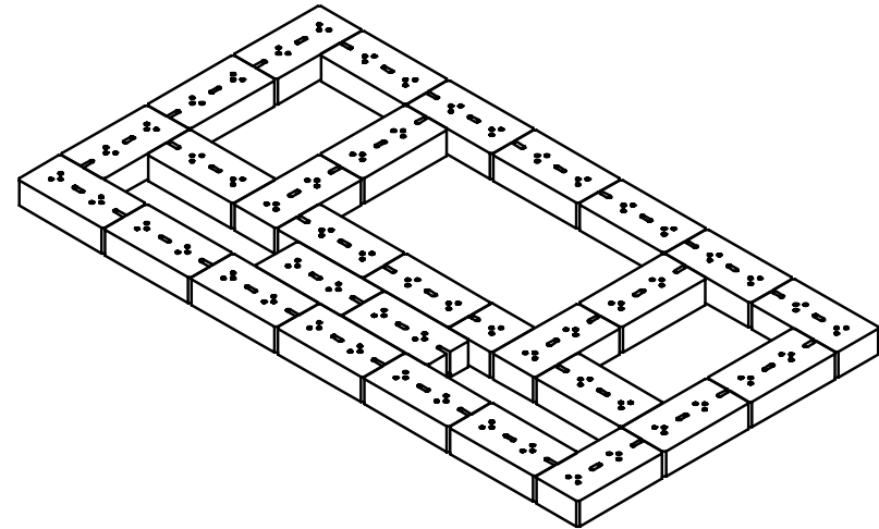
ISOMETRIC VIEW
